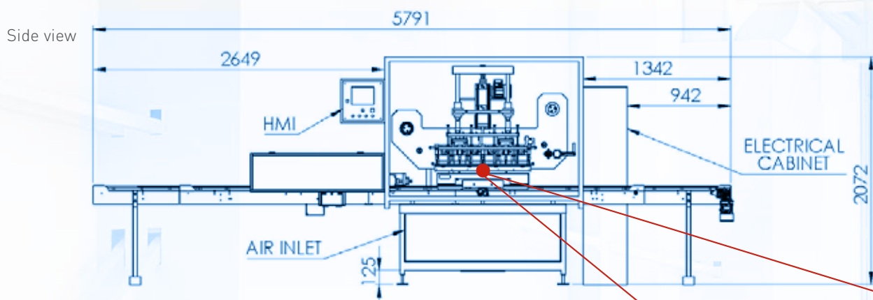
Commanded canisters screw feed registration.
